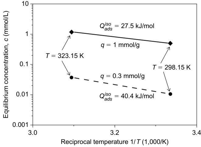
Figure 3.14 Adsorption isotherms for phenol adsorbed onto activated carbon WL2.
