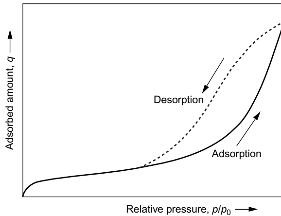
Figure 2.8 Adsorption hysteresis.
